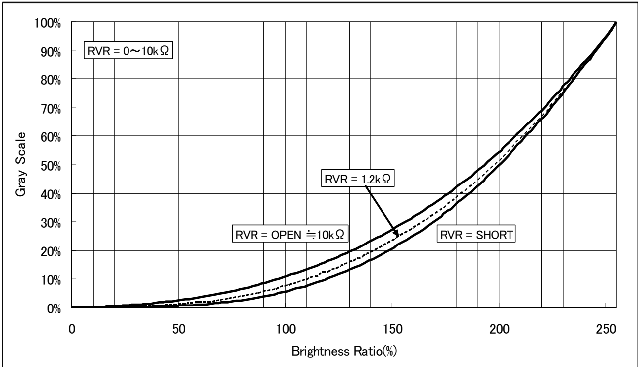
Figure 4-5-1 Gamma characteristics
