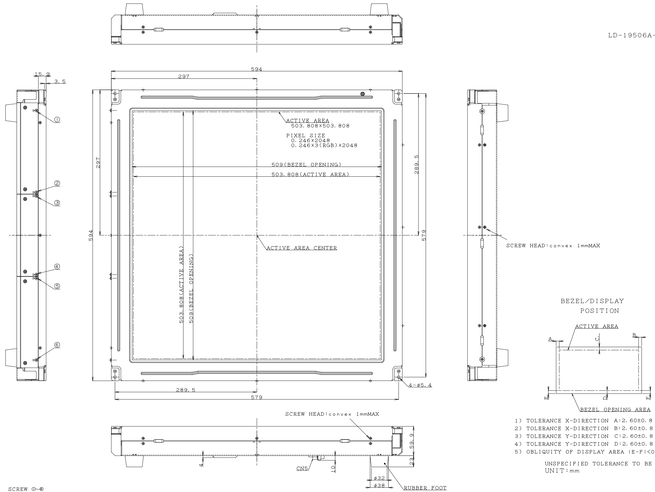
Fig4. LQ281L1LW14 MODULE OUTLINE 1/2
