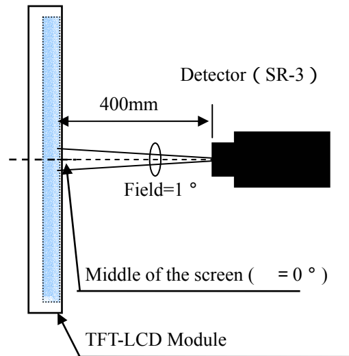
Fig.4-2 Measurement of Contrast, Luminance, Chromaticity and Response time.
