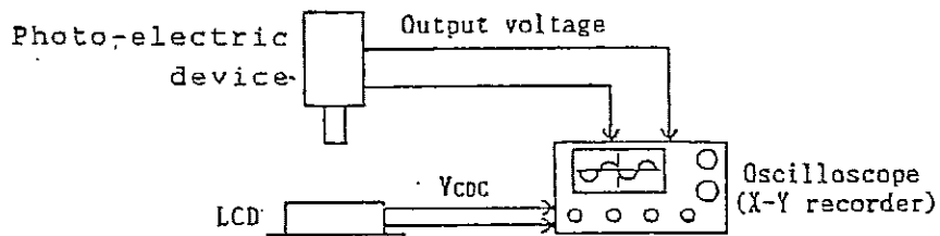
Fig. A Measurement system
