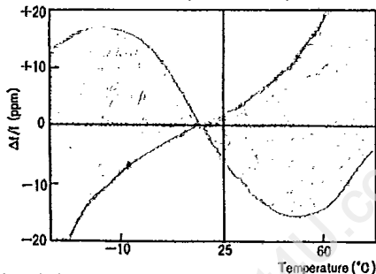
Fig. 5 Temperature - Oscillation Frequency Variation Characteristic (V dd = 5.0V)
