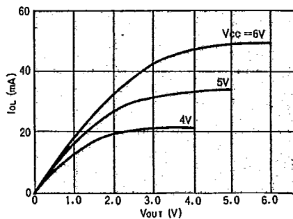
Fig. 6 Example of V out Characteristic (T a = 25°C)
