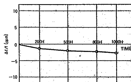
Fig. 8 High Temperature Exposure
