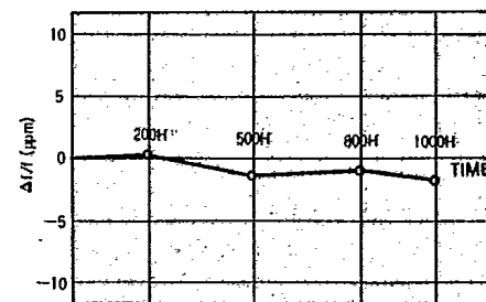
Fig. 9 Low Temperature Exposure Characteristic (T a = 25°C)
