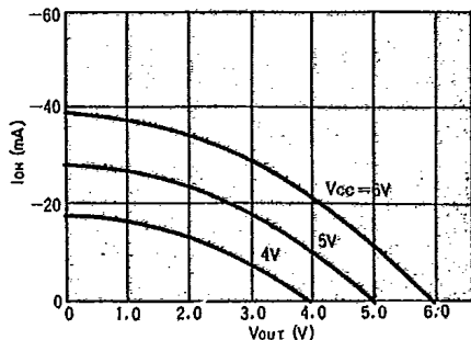
Fig. 7 Example of I oh - V out Characteristic (T a = 25°C)
