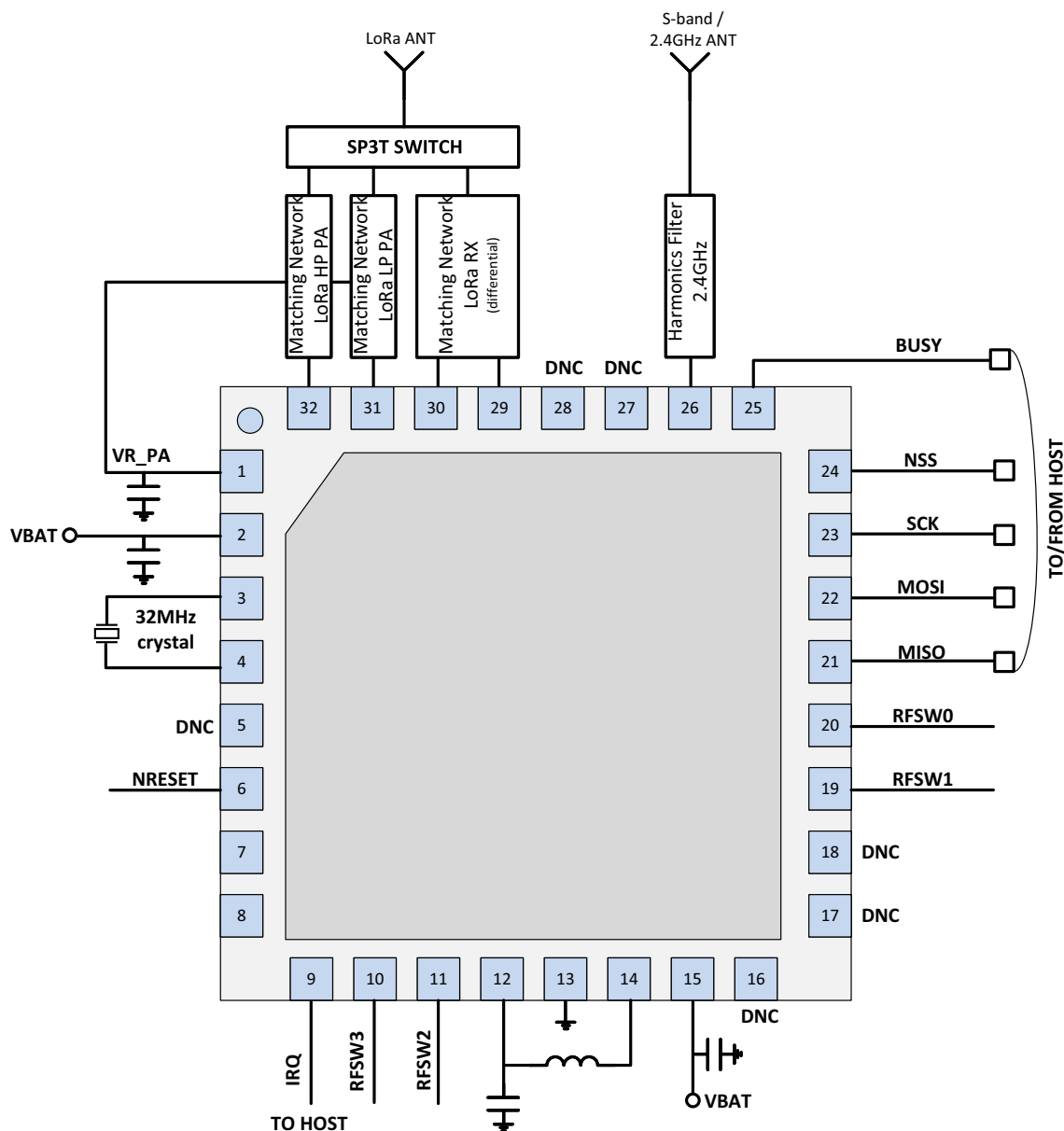
Figure 4-1: Multi-band EU/US LoRaWAN Using Sub-GHz PAs
