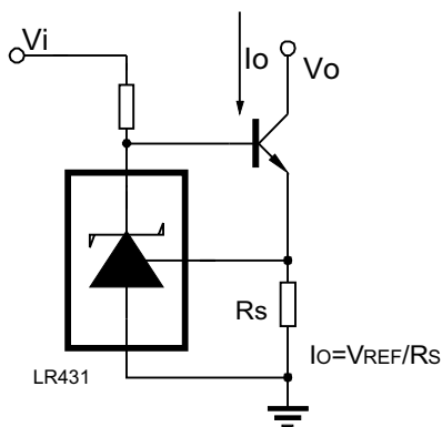
Fig 13 Constant-current Sink
