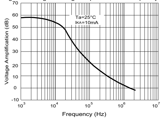
Fig 6 Small Signal Voltage Amplification Vs Frequency
