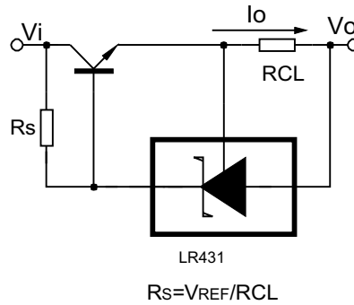
Fig 14 Current Limiting or Current Source
