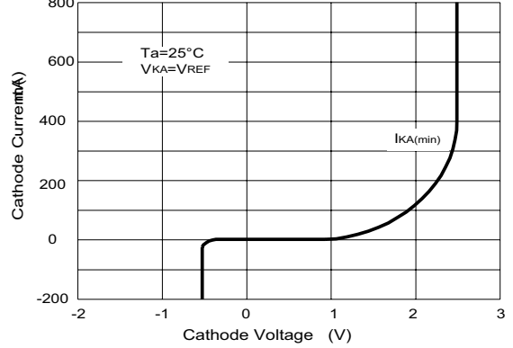
Fig 2 Cathode Current Vs Cathode Voltage
