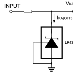
Fig 9 Test Circuit For I_{KA(OFF)}
