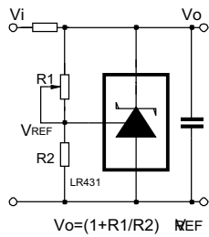
Fig 10 Shutdown Regulator
