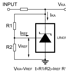
Fig 8 Test Circuit for V_{KA} \geq V_{REF}
