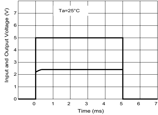
Fig 4 Pulse Response
