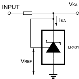
Fig 7 Test Circuit For V_{KA}=V_{REF}
