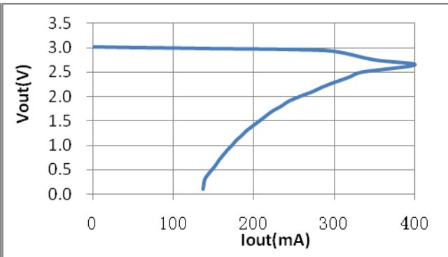
6. Current limit
