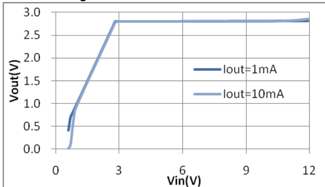
2. Line regulation
