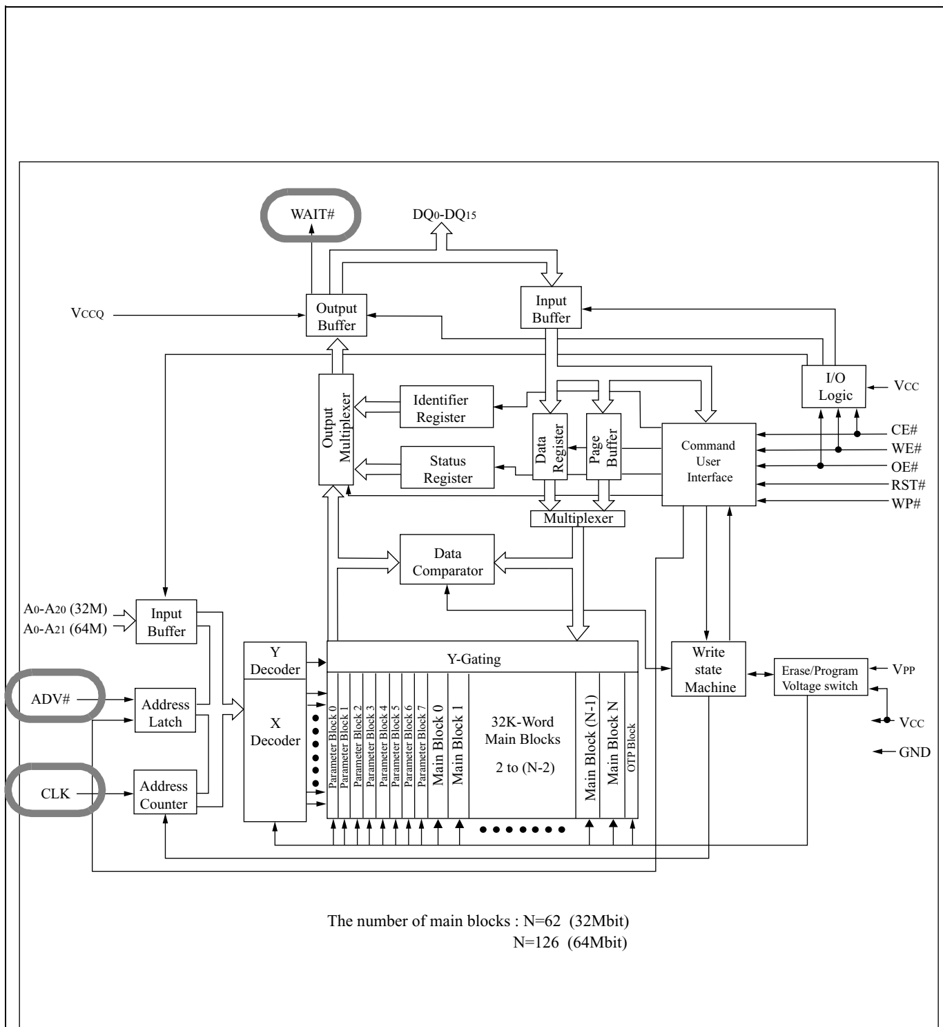
Figure 1. Block Diagram
