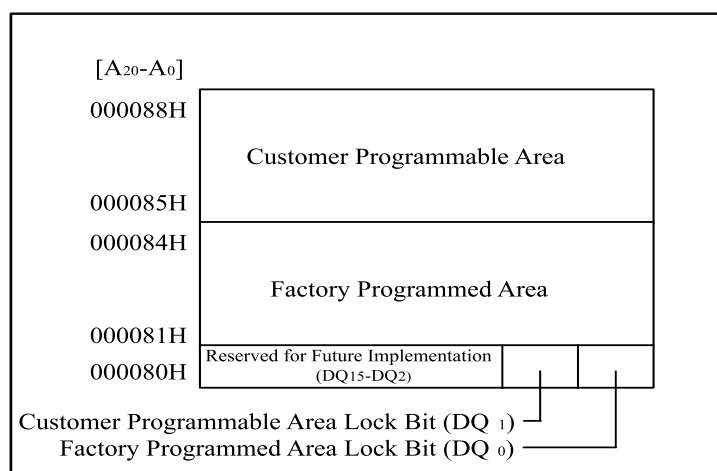
OTP Block Address Map for OTP Program (The area outside 80H - 88H cannot be used.)
