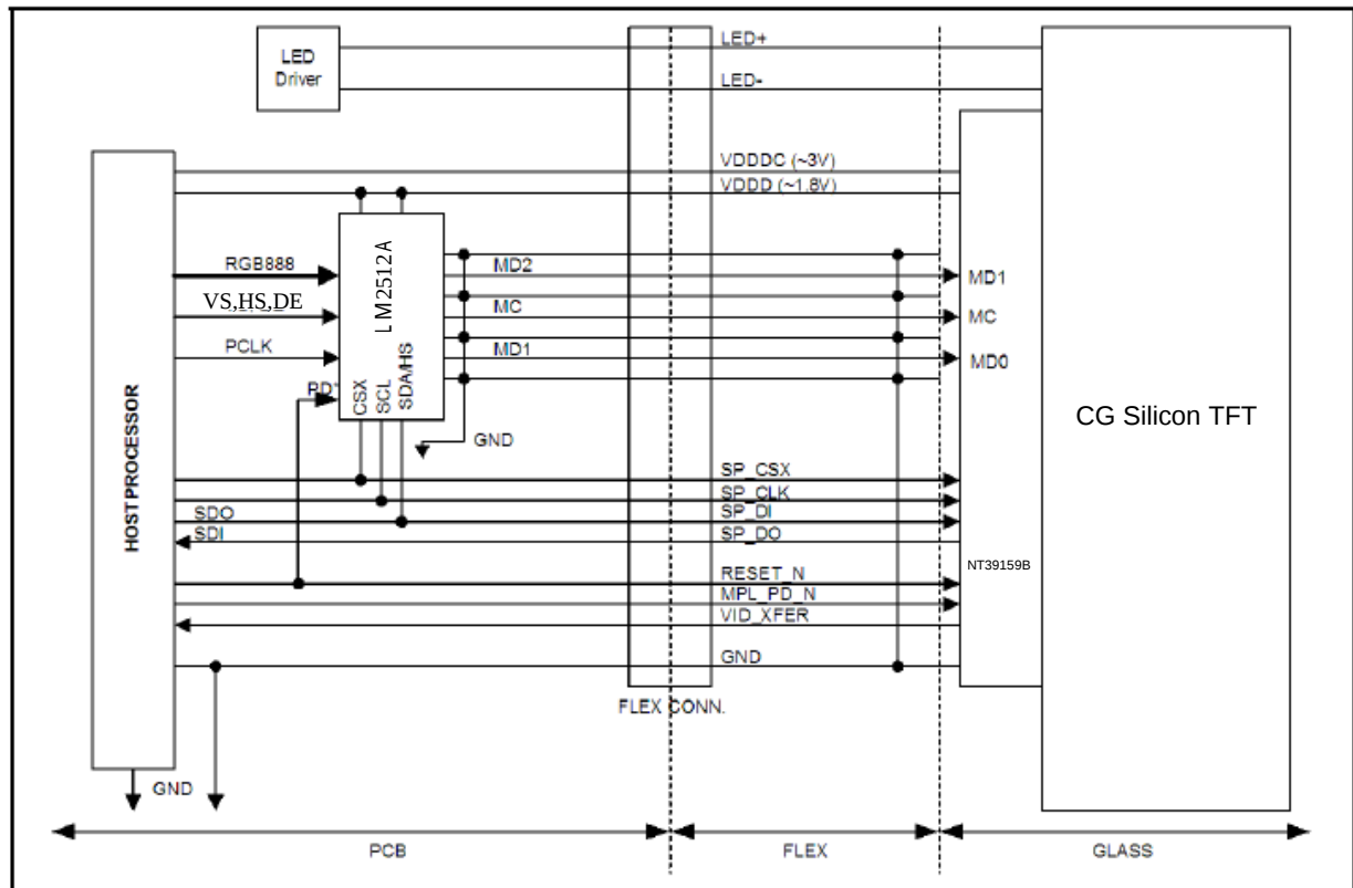
Figure1. MPL1 signal connections
