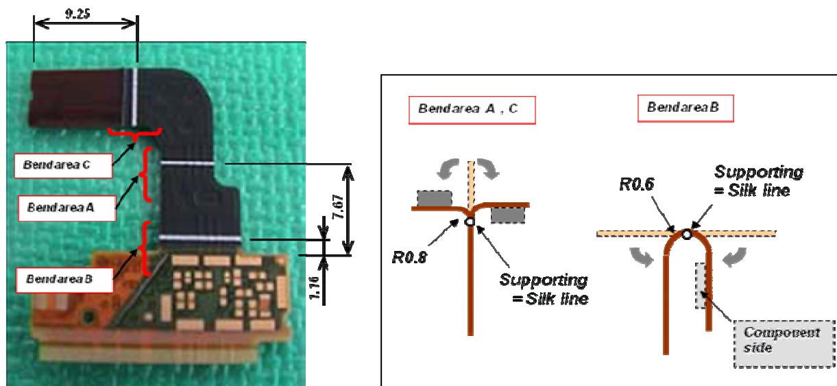
Figure16. FPC bending Area (A,B,C)
