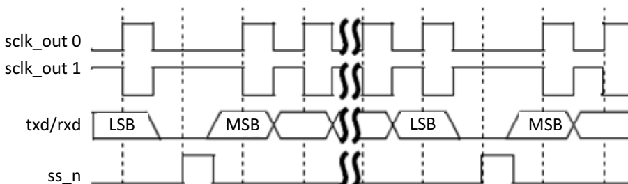
Figure 9-4 SPI Serial Format Continuous Transfers (SCPH = 0)
