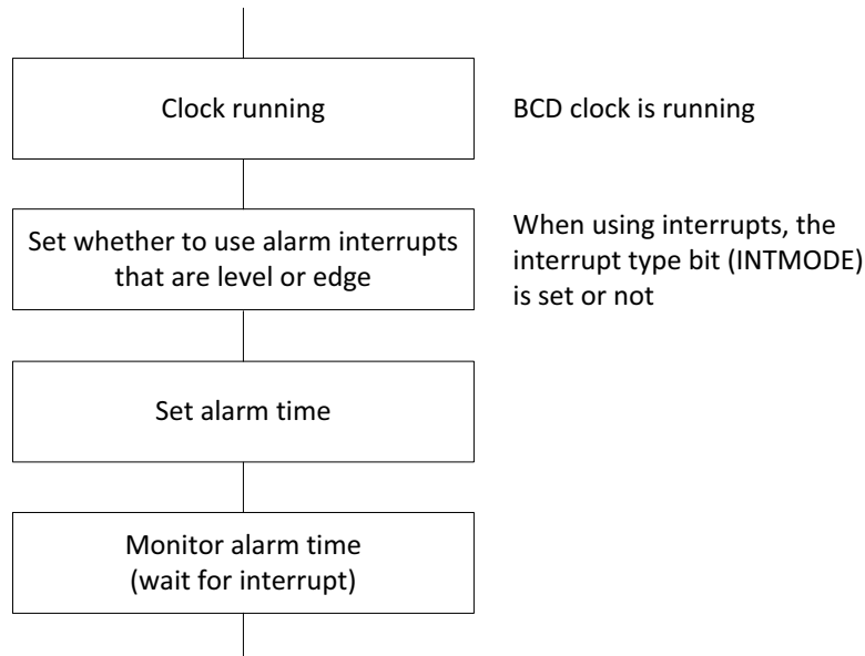
Figure 8-3 Alarm Functions
