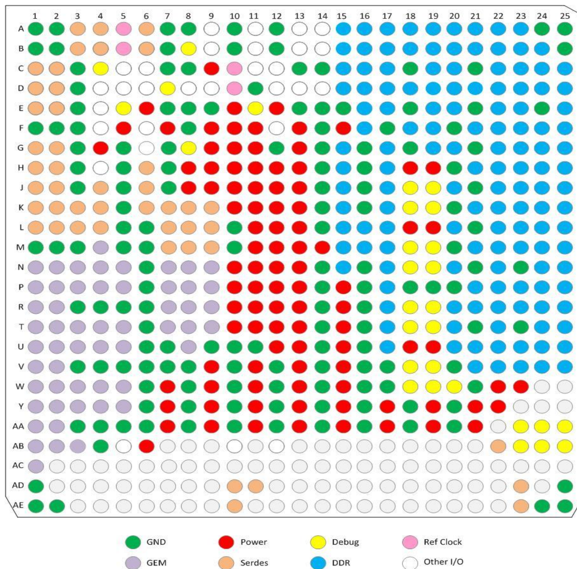
Figure 3-1 LS1024A Ball Map
