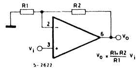
Fig. 18 - Non-inverting amplifier
