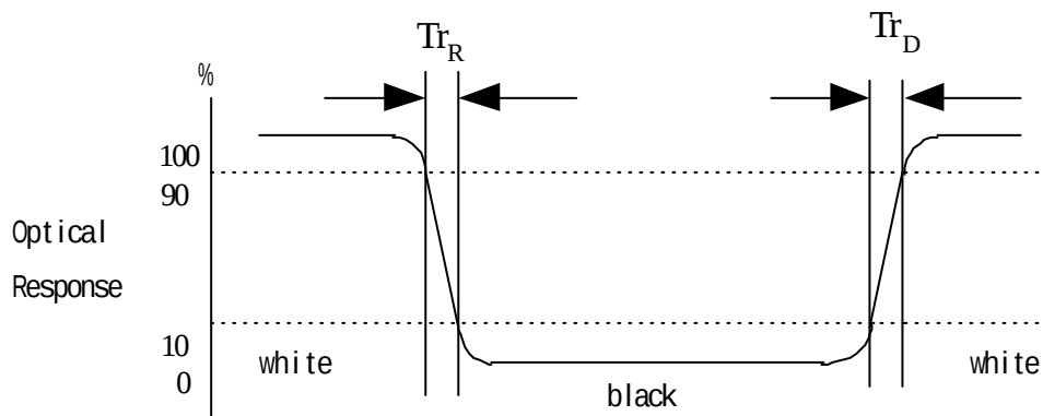
FIG. 4 Response Time
