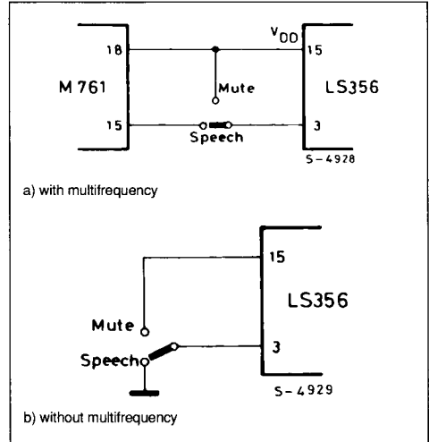
Figure 15 : External Mute Function.
