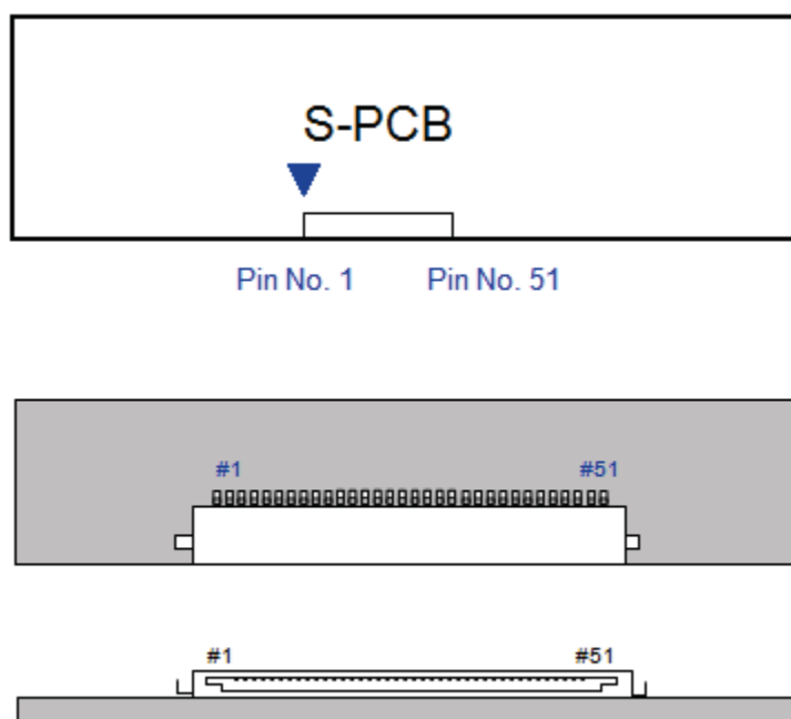
Fig. Connector diagram
