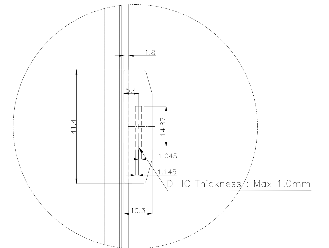
DETAIL "B"(HIDDEN VIEW) (3 : 1)
