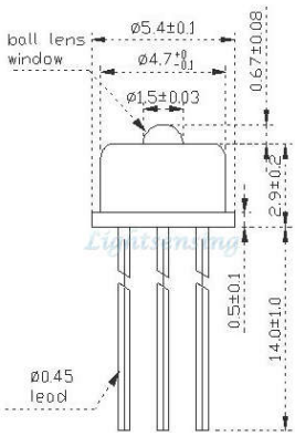
Short ball lens TO Model: S1
