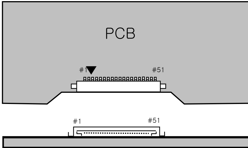
Fig. Connector diagram
