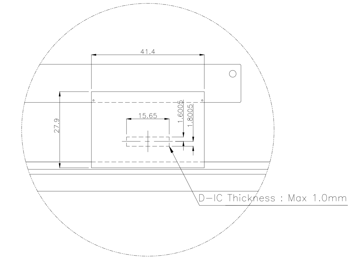
DETAIL "A" (3 : 1)
