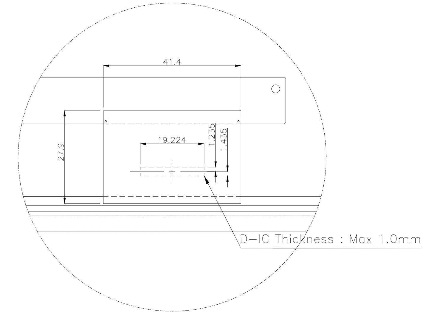
DETAIL "A" (3 : 1)
