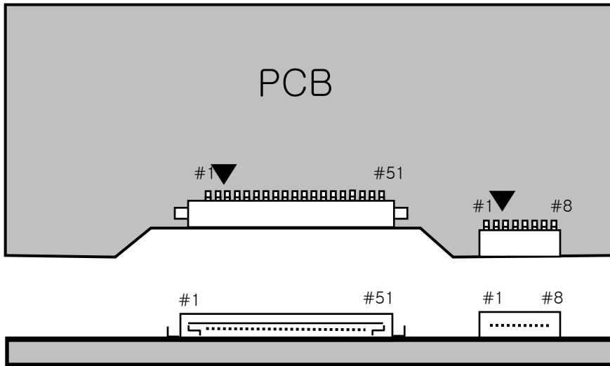
Fig. Connector diagram
