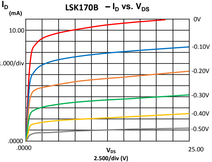
Output Characteristics
