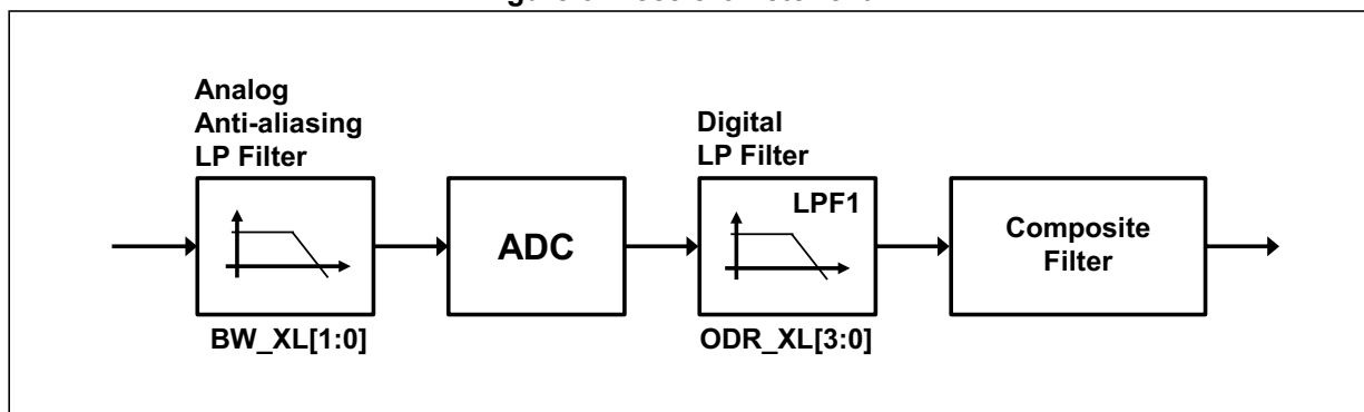
Figure 6. Accelerometer chain
