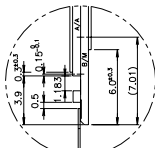
DETAIL "D" (SCALE 5:1)
