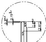
DETAIL "C" (SCALE 5:1)
