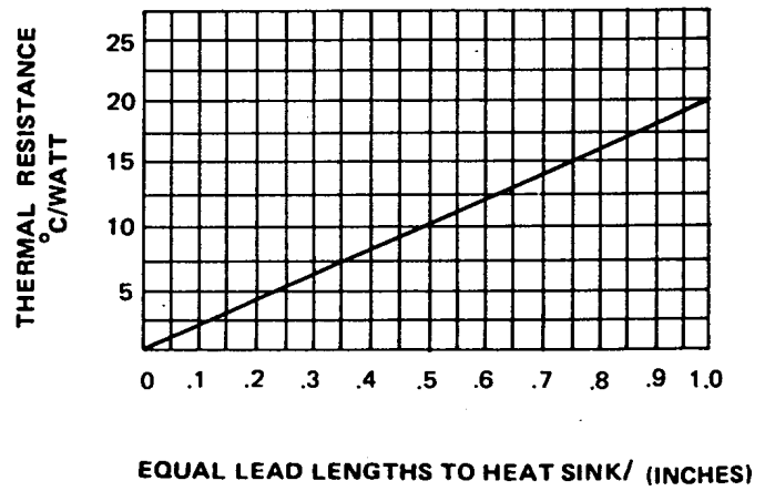
FIG. 4-TYPICAL THERMAL RESISTANCE
