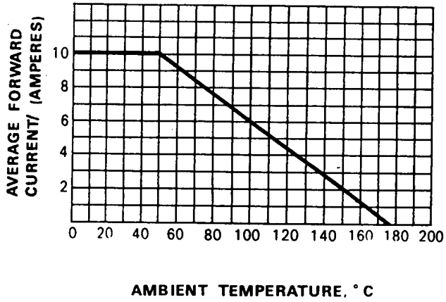
FIG. 1-FORWARD DERATING CURVE
