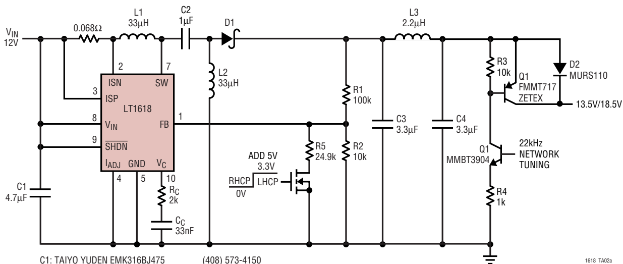
4.5W Direct Broadcast Satellite (DBS) Power Supply with Short-Circuit Protection
