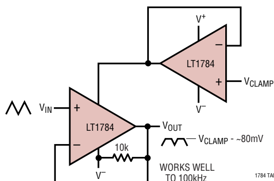
Adjustable Clamp
