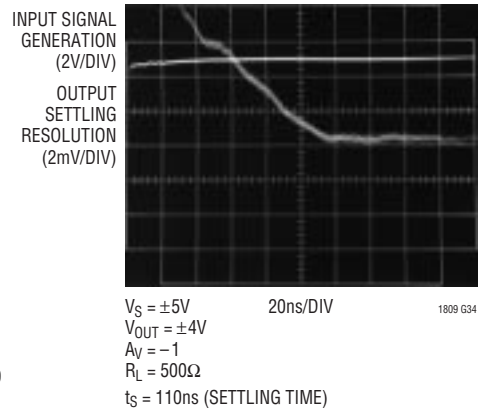
0.01% Settling Time
