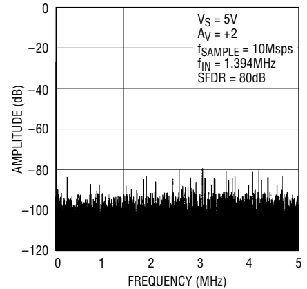
Figure 7. 4096 Point FFT Response
