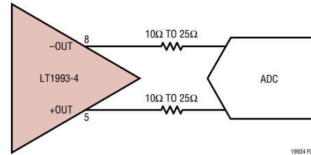
Figure 4. Adding Small Series R at LT1993-4 Output
