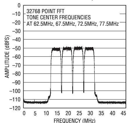
4-Tone WCDMA Waveform LT1993-4 Driving LTC2255 14-Bit ADC at 92.16Mps
