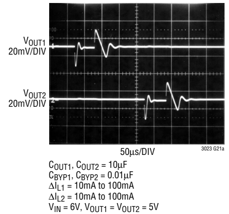
Channel-to-Channel Isolation
