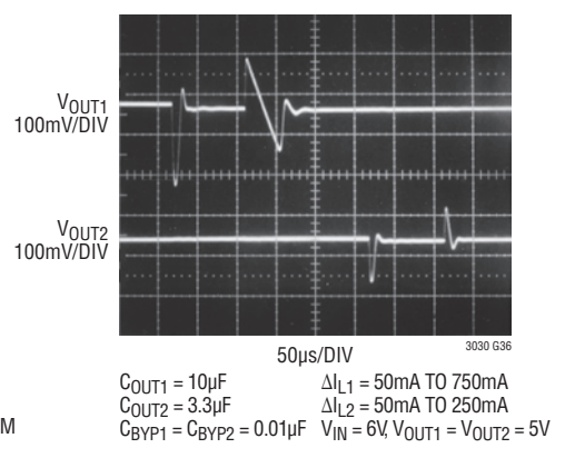
Channel-to-Channel Isolation
