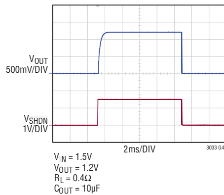
SHDN Transient Response C_{REF/BYP} = 10\text{nF}
