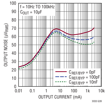
RMS Output Noise V_{OUT} = 0.2\text{V}, C_{FF} = 0
