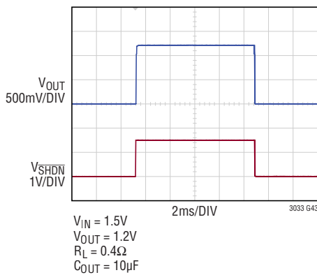
SHDN Transient Response C_{REF/BYP} = 0
