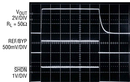
SHDN Transient Response C_{REF/BYP} = 0
