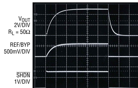
SHDN Transient Response C_{REF/BYP} = 10\text{nF}
