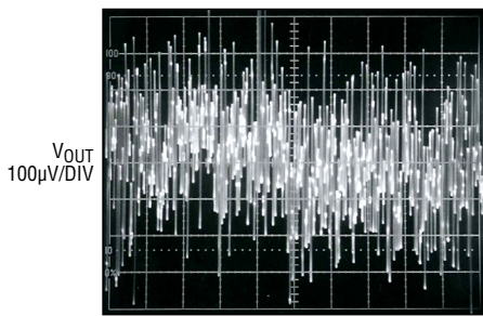
5V 10Hz to 100kHz Output Noise C_{REF/BYP} = 10\text{nF}, C_{FF} = 0
