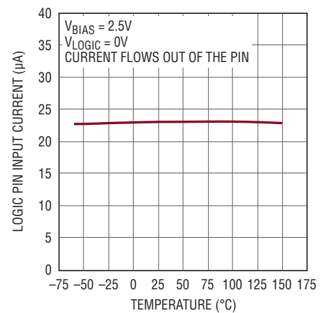
Logic Pin Input Current, Low State
