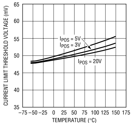
Current Limit Threshold Voltage vs Temperature
