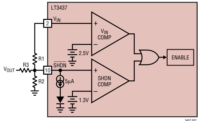
Figure 7. Undervoltage Lockout
