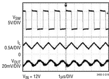
Operating Waveforms
