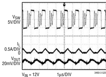
Operating Waveforms, Discontinuous Mode
