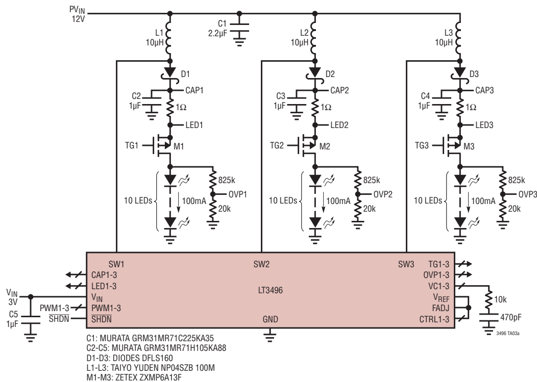
Triple Boost 100mA × 10 LED Driver
