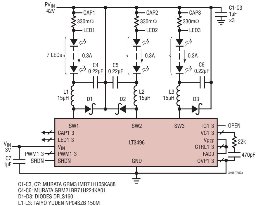
Minimum BOM Buck Mode LED Driver
