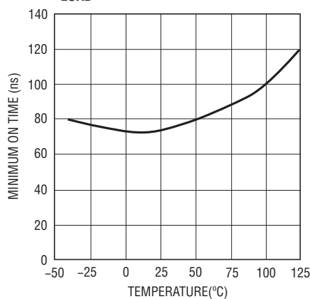
Min ON Time vs. Temperature I_{LOAD} = 0.3A
