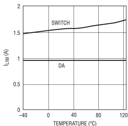
I_{LIM} vs Temperature
