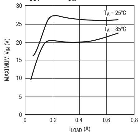
Max V_{IN} for Constant Frequency V_{OUT} = 3.3V , f_{SW} = 2MHz
