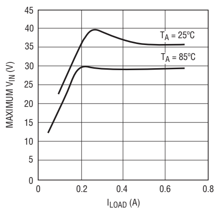
Max V_{IN} for Constant Frequency V_{OUT} = 5V , f_{SW} = 2MHz
