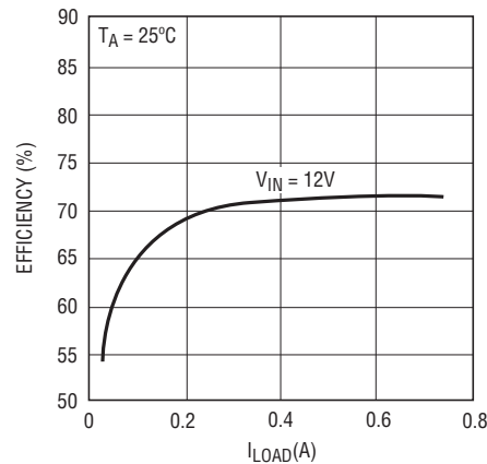
Efficiency vs Load Current V_{OUT} = 1.8V , f_{SW} = 0.7MHz
