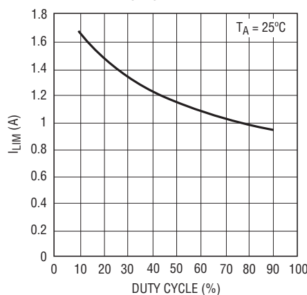
I_{LIM} vs Duty Cycle
