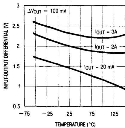
Dropout Voltage
