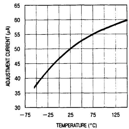
Adjustment Current
