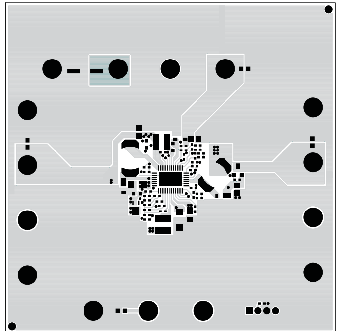
Figure 4. Topside PCB Layout
