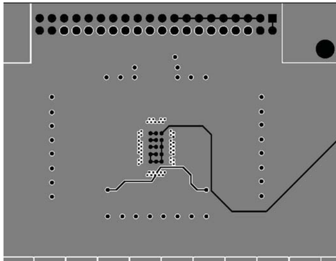
Figure 7. PCB Layer 4
