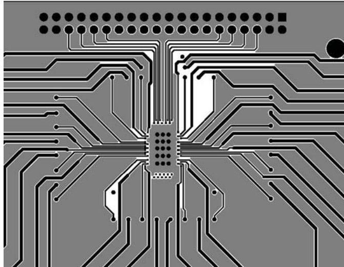
Figure 6. PCB Layer 3
