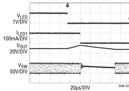
LED Open-Fault Waveforms
