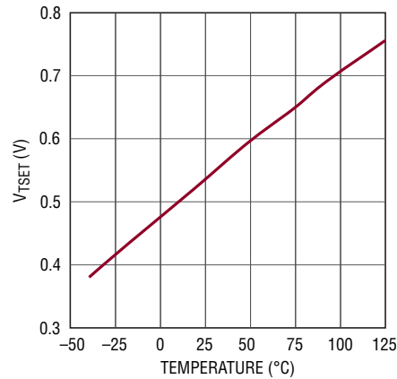
V_{\text{TSET}} for LED Current Derating
