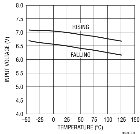
Undervoltage Lockout
