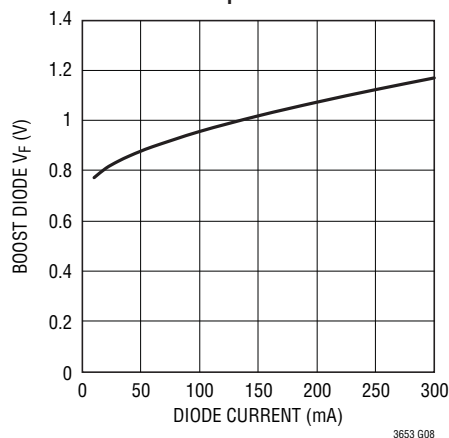
Boost Diode V_F
