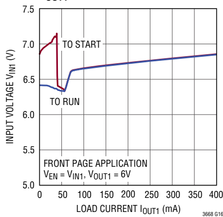
Minimum Input Voltage, V_{OUT1} = 6V
