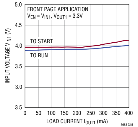
Minimum Input Voltage, V_{OUT1} = 3.3V
