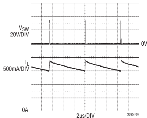
Figure 7. The LT3695 Reduces its Frequency to Protect Against Shorted Output with 36\text{V} Input
