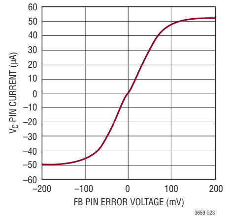
Error Amplifier Output Current
