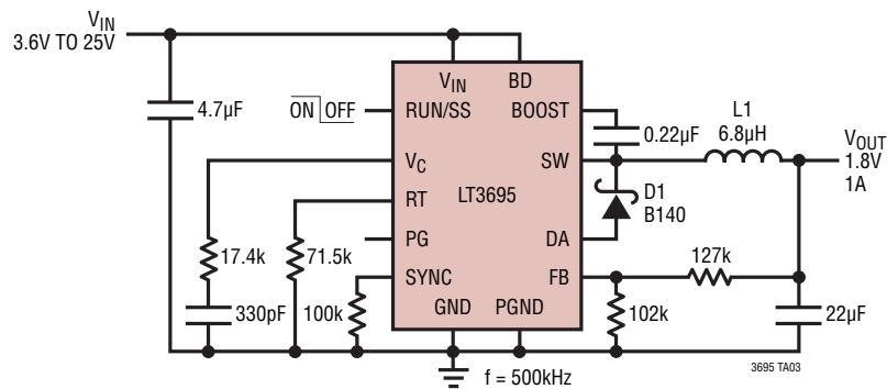
1.8V Step-Down Converter
