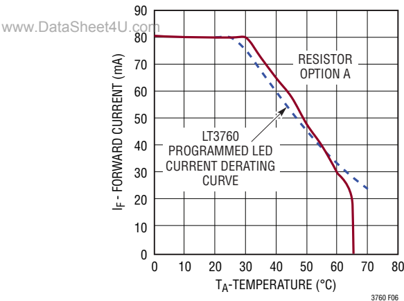
Figure 6. LED Current Derating vs LED Ambient Temperature
