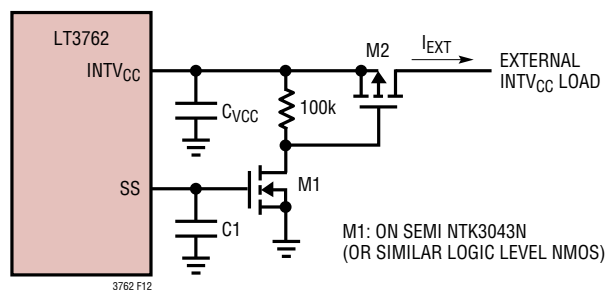
Figure 12. Powering External Circuits with INTV_{CC}
