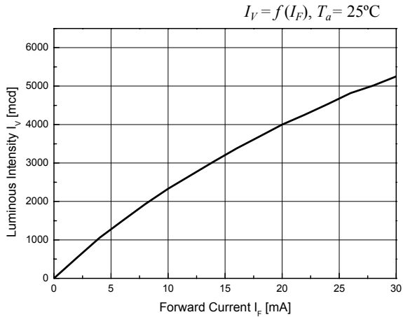
Forward Current vs. Luminous Intensity vs.
