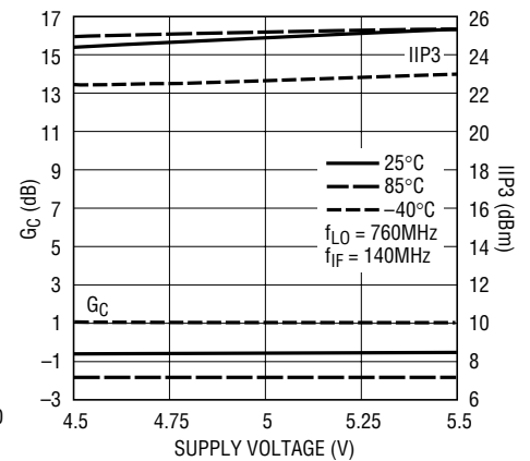
Low Band Conv Gain and IIP3 vs Supply Voltage (RF = 900MHz)
