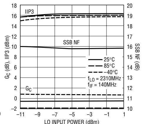
High Band Conv Gain, IIP3 and SSB NF vs LO Power (RF = 2450MHz)
